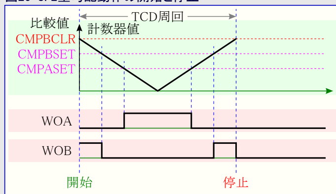
図25-8. 2重勾配動作の開始と停止 (Start and Stop of Double Slope Operation)
