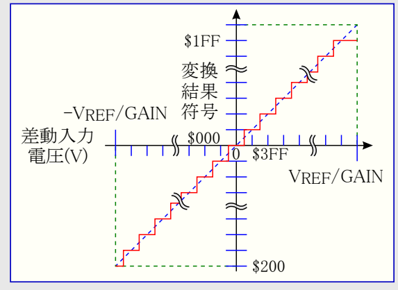
図28-12. 差動入力計測範囲
