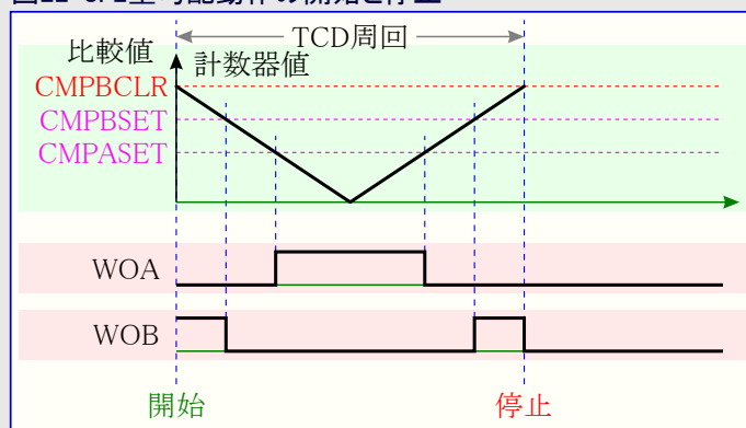
図22-8. 2重勾配動作の開始と停止 (Start and Stop of Double Slope Operation)
